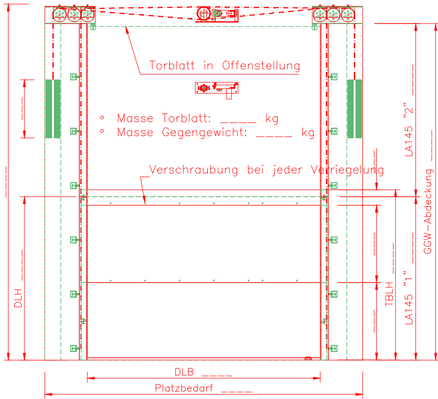
DETAIL "A" M=2,5:1
